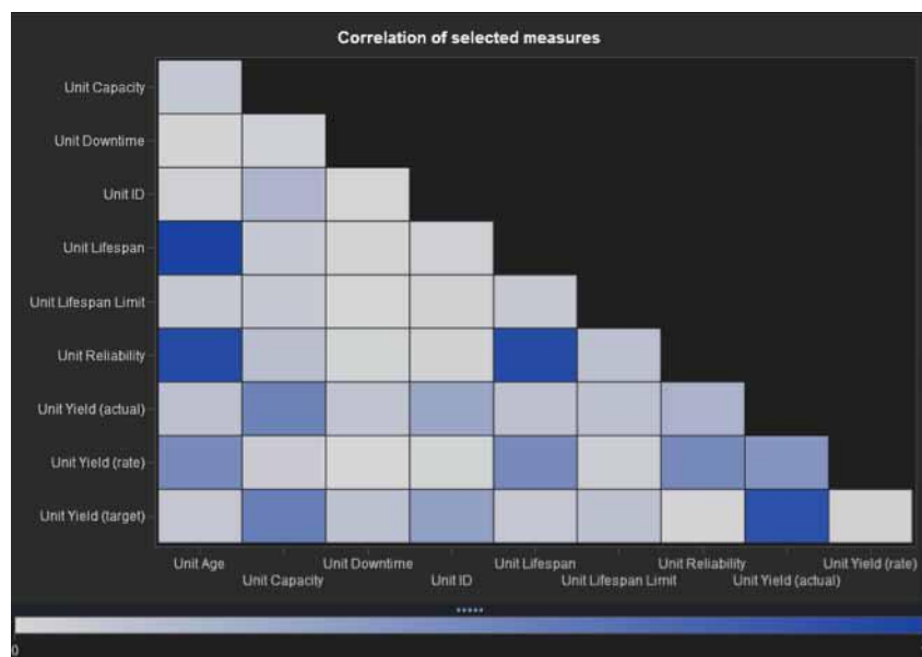
Figure 11: In this autocharted correlation matrix, darker boxes indicate a stronger correlation; lighter boxes indicate a weaker correlation. You can double-click on a box for further details.
